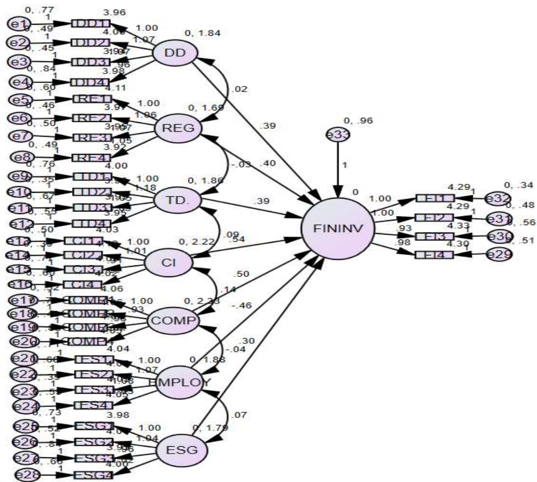
Fig. 2. Structural Model with Estimates
